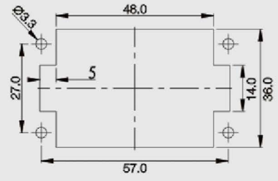
面板安装开孔图 Panel cut out
